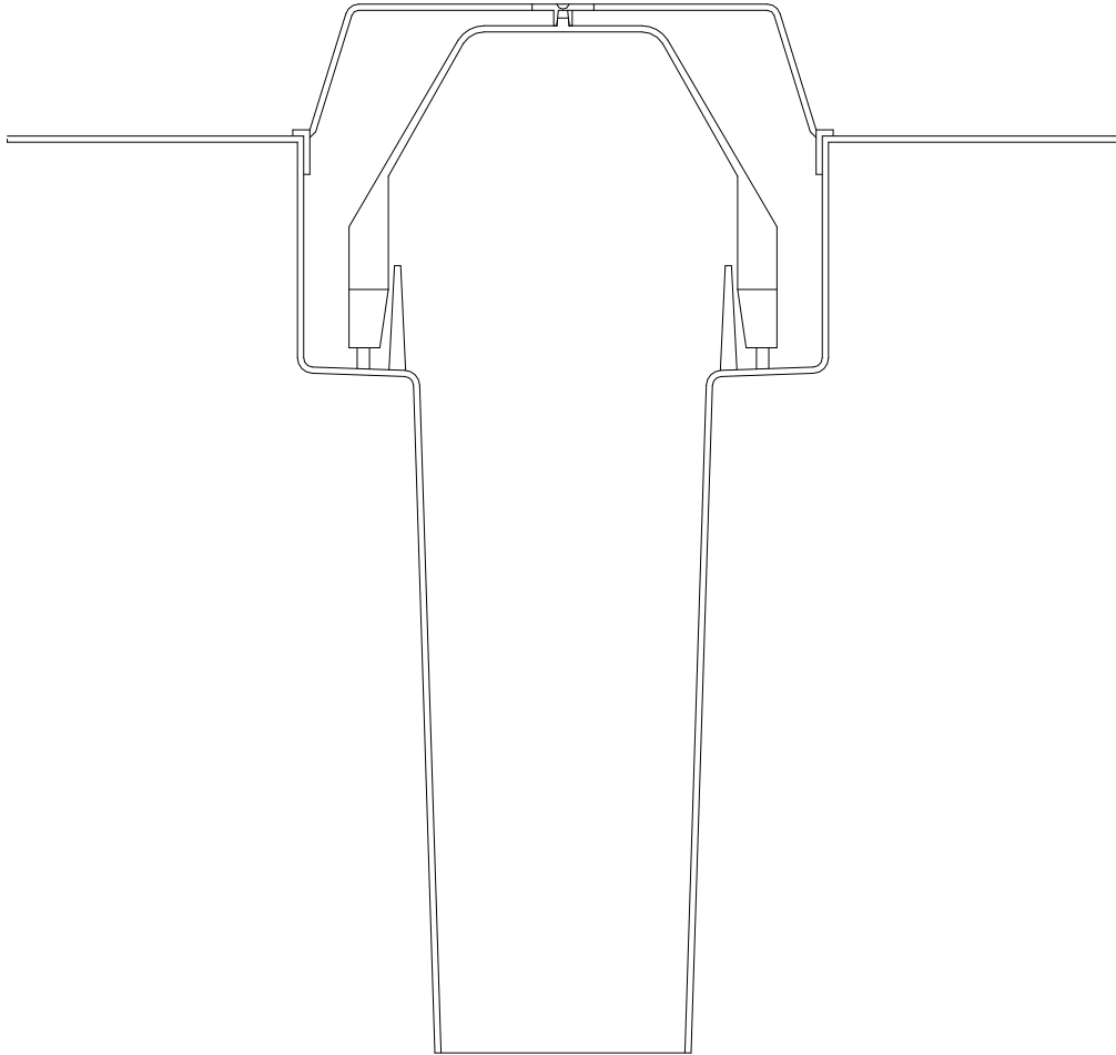
WALLBARN LIMITED BITUMINOUS MEMBRANES SECTION OF EPDM DRAIN OUTLET WITH SIPHON (SIZE SHOWN \phi 90\text{mm} X 250\text{mm} )
